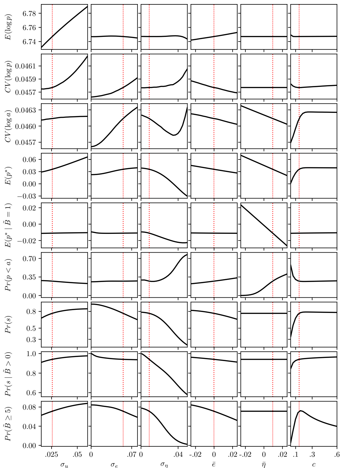
Figure 6: Moment comparative statics.
