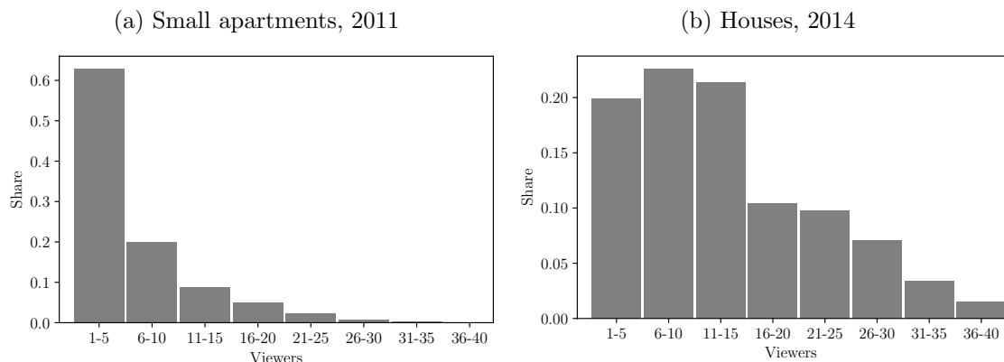
Figure 5: Empirical viewer distribution.
