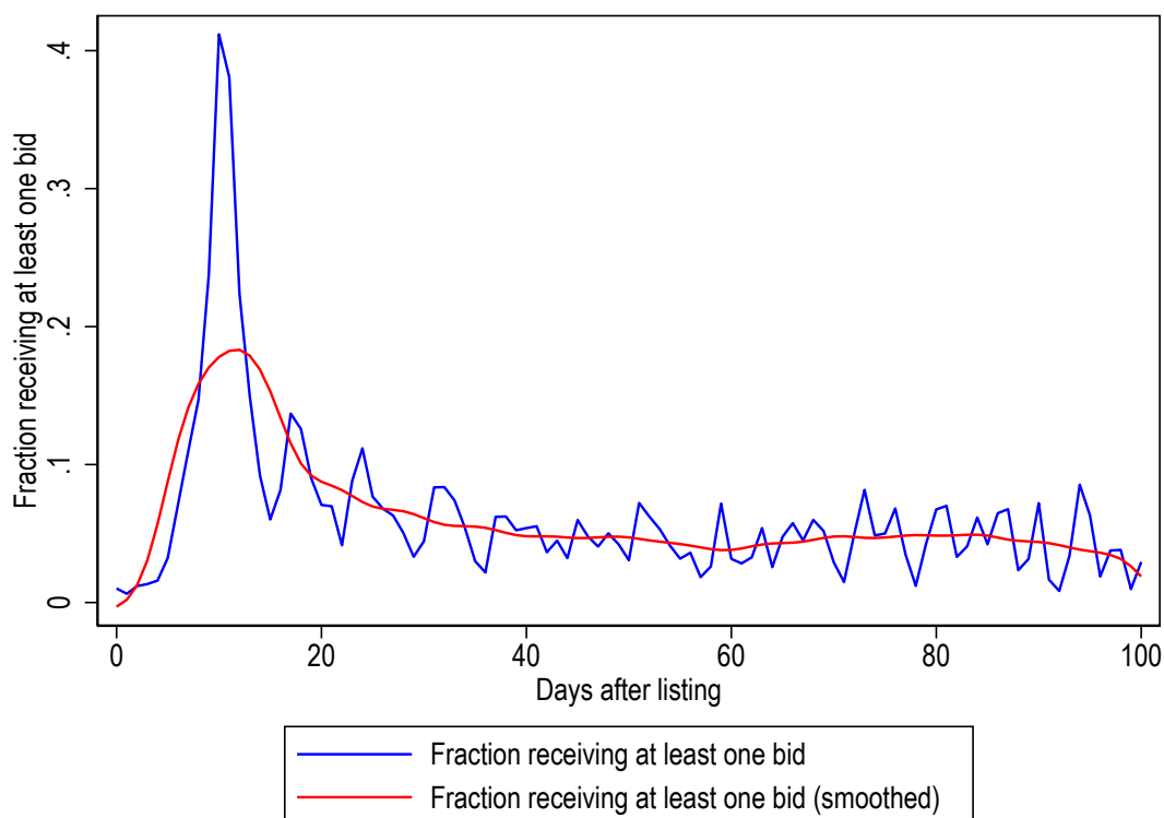
Figure 3: Bidding hazard.
