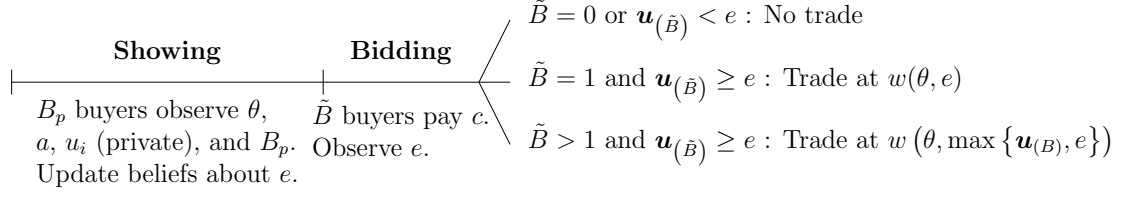
Figure 1: Model time-line.
