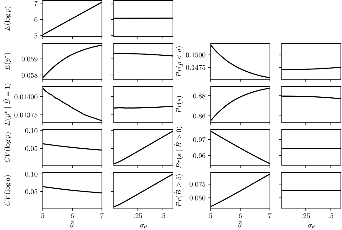
Figure 7: Moment comparative statics for \bar{\theta} and \sigma_\theta .
