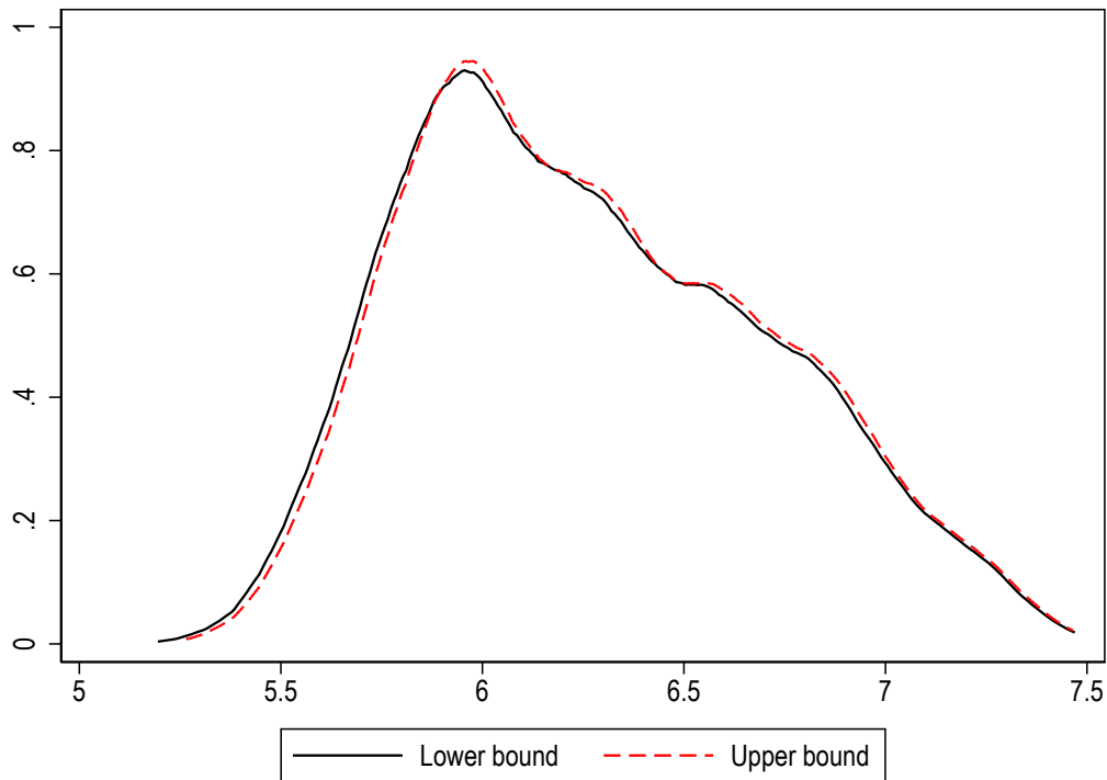
Figure 8: Losing bidder valuations.
