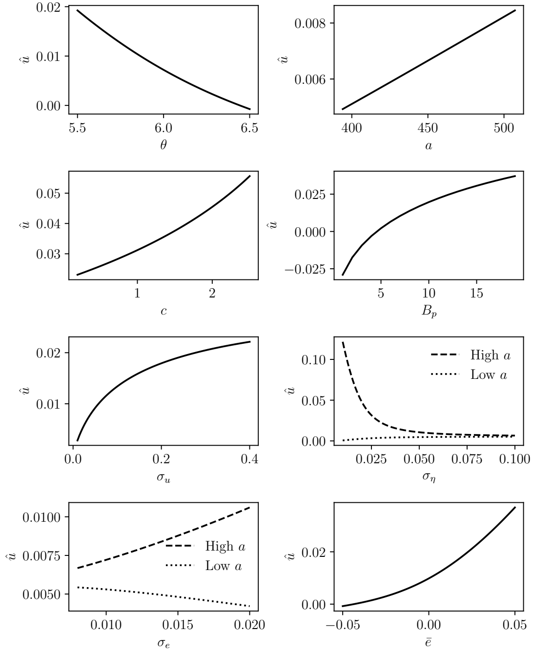
Figure 2: Comparative statics for \hat{u} .
